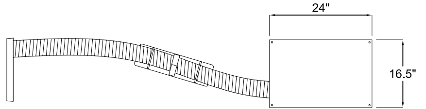
TOP VIEW
