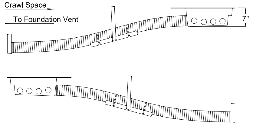
SIDE VIEWS
