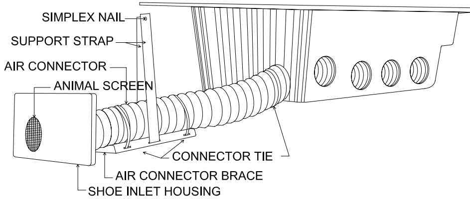
INSTALLED VIEW
